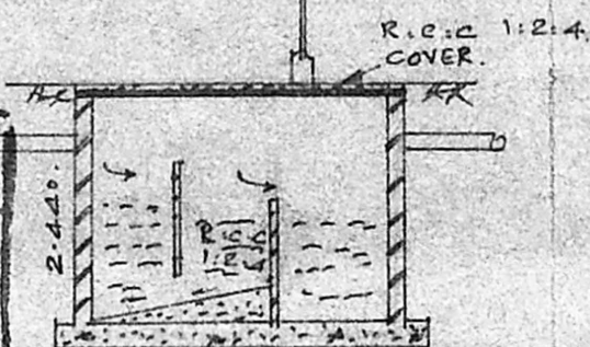
SECTION OF S.T.
